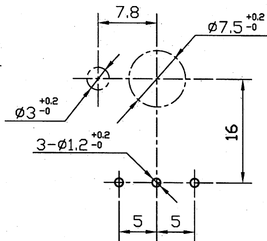
MOUNTING HOLE DETAIL (VIEWPOINT OF SHAFT)
